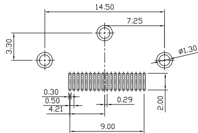
RECOMMENED P.C.B LAYOUT(t=1.6mm) TOLERANCES UNLESS OTHERWISE SPEC.±0.05
