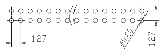
Recommended P.C.B Layout(Top Side) (PCB BOARD TOLERANCE±0.05)
