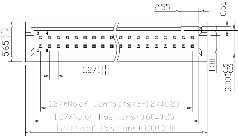
Recommended P.C.B Layout(Top Side) (PCB BOARD TOLERANCE±0.05)
