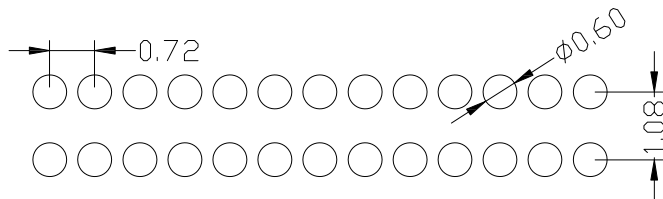
PCB LAYOUT
