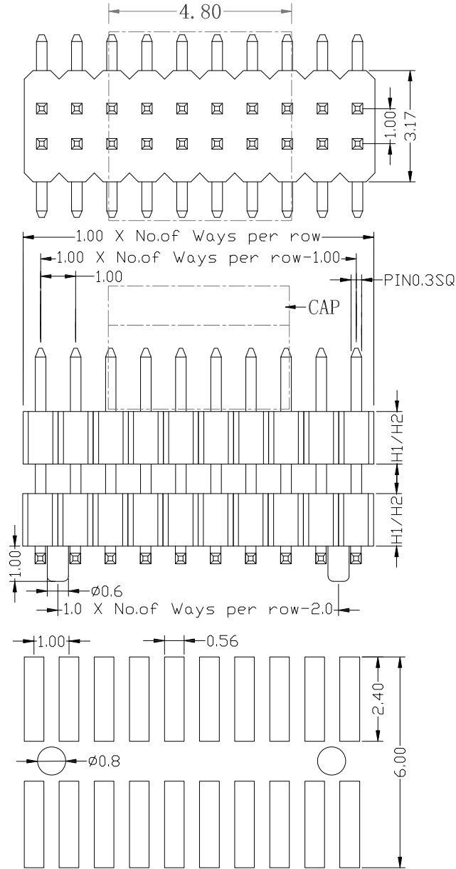
PCB LAYOUT
