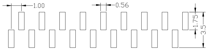
PCB LAYOUT
