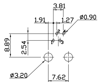
PCBLAYOUT (TOPView)
