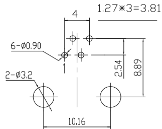
PC BOARD LAYOUT THICKNESS=1.6MM
