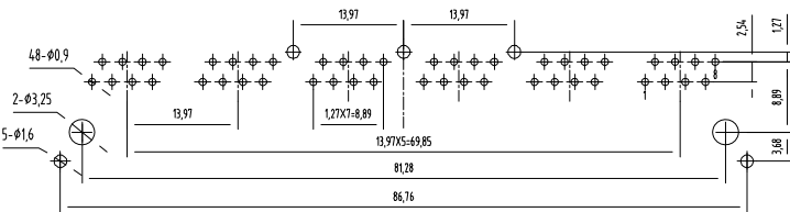
PC Board Layout Component Side Shown
